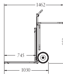
GS-Compact 800 R
