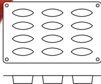
14.10056 SF038 12 medium boat, 20 ml (7,2x3 cm | 1,5 cm) 17,3x29,7 cm pack: 1
